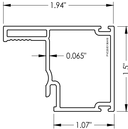
8 DSL MAIN SASH
