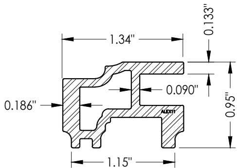
15 REINFORCEMENT
