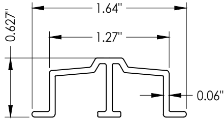
11 ANTLIFT TRACK
