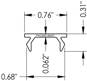
10 DSL COVER
