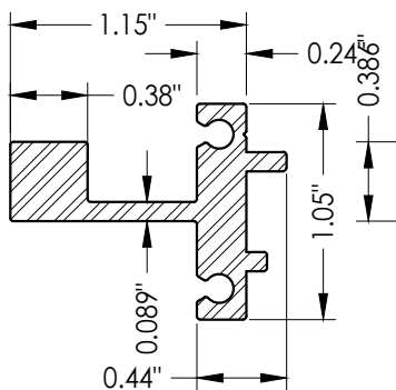
14 REINFORCEMENT
