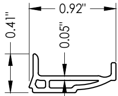
9 GLAZING BEAD
