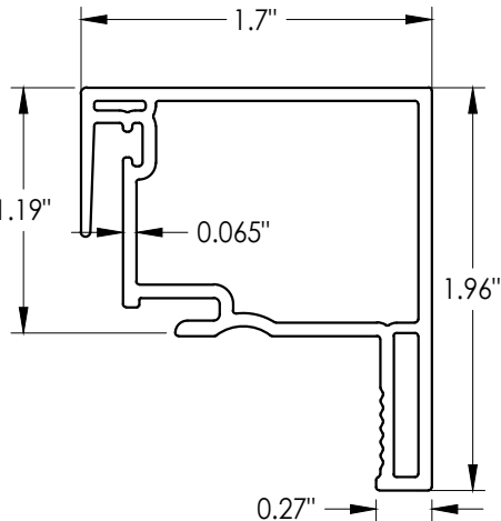
7 LOCK RAIL
