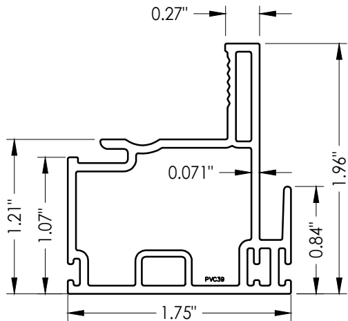
6 KEEPER RAIL
